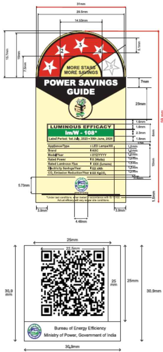
Dimension of the label and QR code to be stamped on the lamp:
