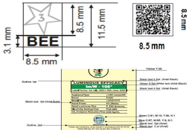
Dimension of the label and QR code to be stamped on the lamp:
