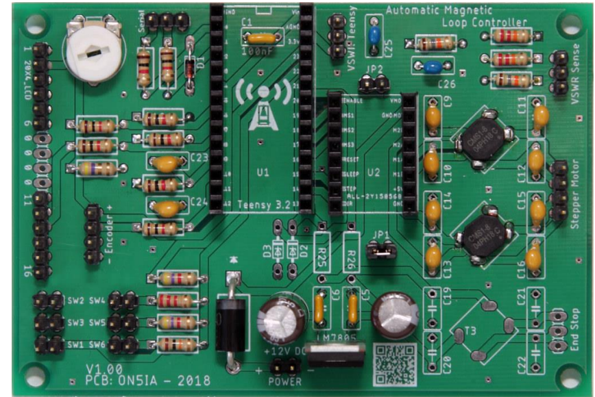
Populated PCB or PCB assembly (PCBA) :
